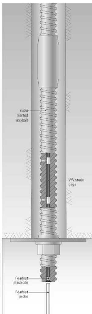
Figure 1 Model 4910 Installation
