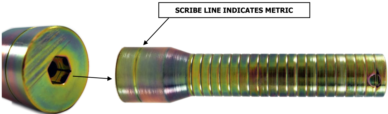
Figure 11: Tab Removal Tool (TRT)
