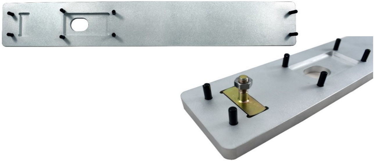
Figure 15: ST350 Extension Mounting Jig
