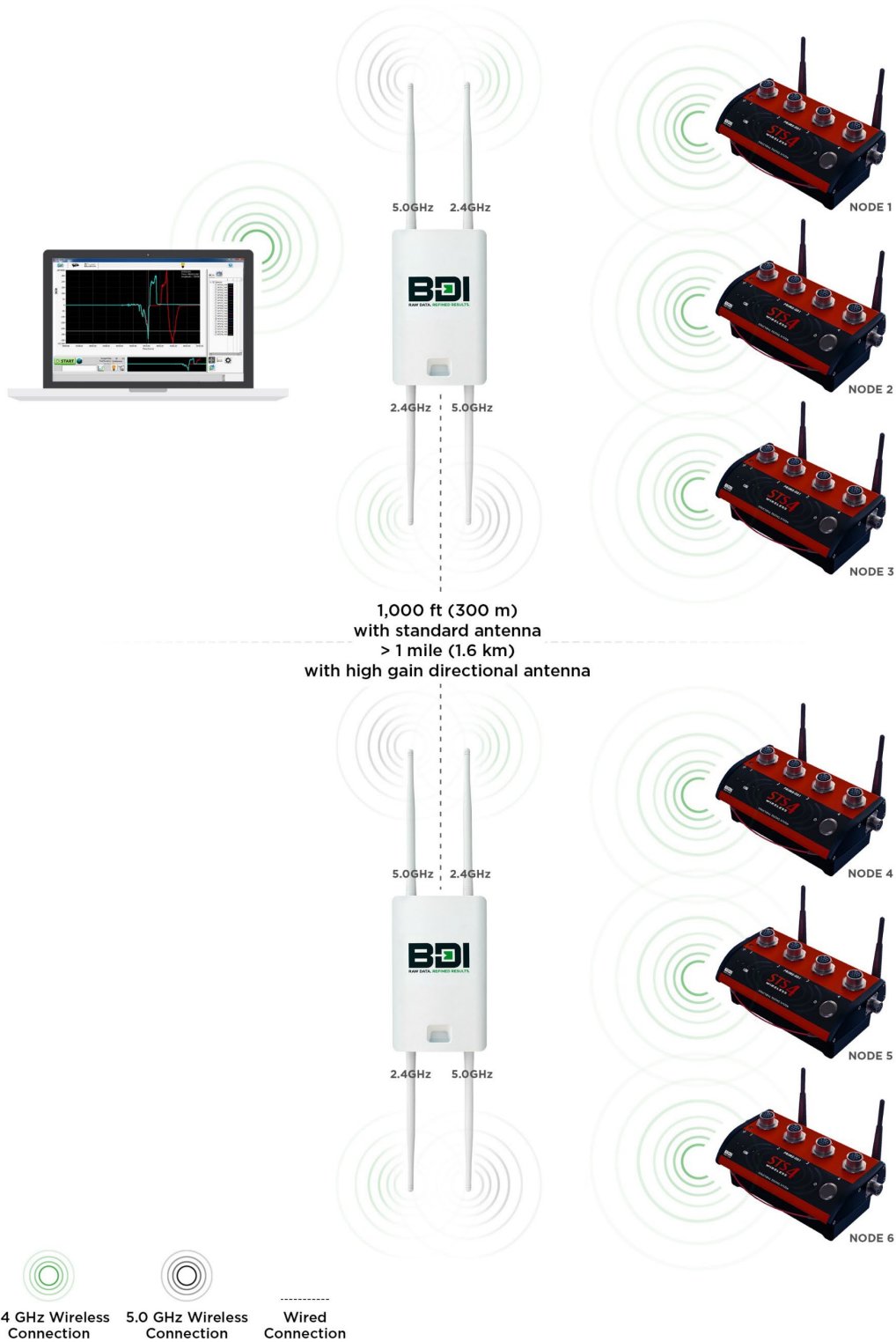
Figure 13: 100% Wireless Multiple STS4-WBS
