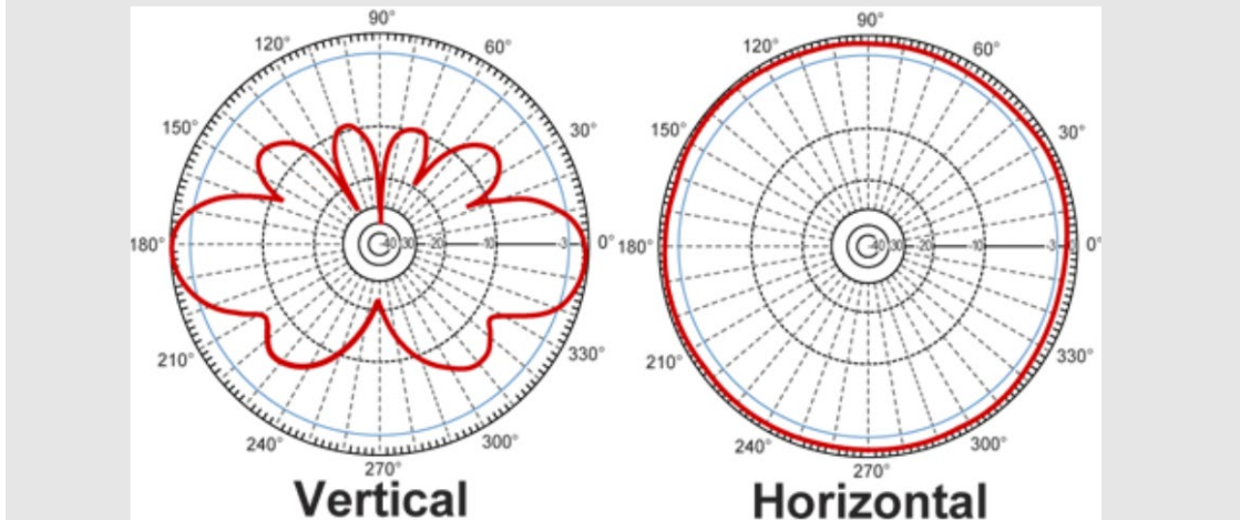
Figure 14: Wireless radiation pattern for typical omni-directional antennas
