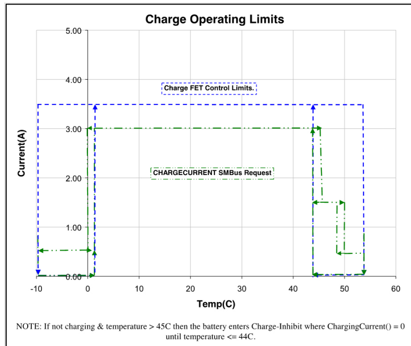
Figure 7: Battery Charging Operating Limits (Courtesy Inspired Energy, LLC)
